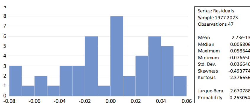
Figure 2. Normality Assessment: Jarque-Bera Test
