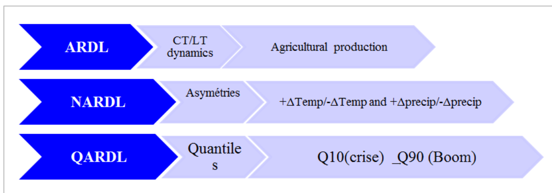
Figure 1. ARDL, NARDL, QARDL: Agricultural Production Modeling Approaches.
