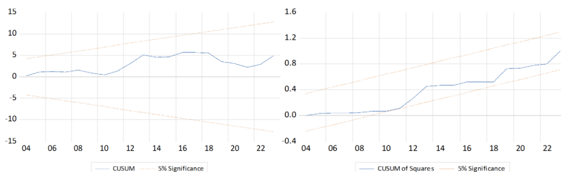
Figure 3. CUSUM / CUSUM 2 Plots.
