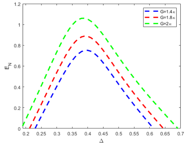
Figure 2. Plots of entanglement E_N versus detuning \Delta/\omega for L = 3 \text{ mm} , \omega_m = 2\pi \times 10^7 \text{ Hz} , \gamma = 2\pi \times 100 \text{ Hz} , T = 100 \times 10^{-3} \text{ K} , \lambda = 810 \times 10^{-9} \text{ m} , c = 3 \times 10^8 \text{ m/s} , P = 10 \text{ mW} , f = 1.07 \times 10^4 and for different values of parametric gain of OPA \gamma .
