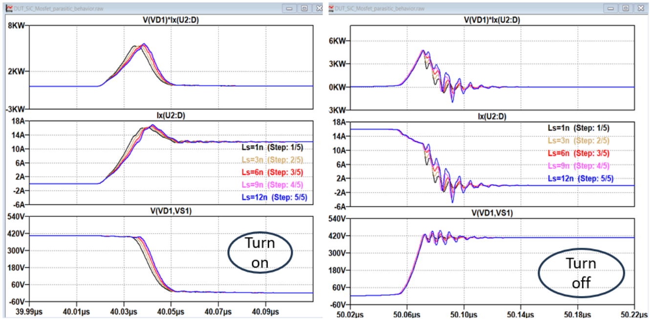
Figure 17. Voltage, current and power loss curves of the transistor during switching (on/off) operation for different L_s values.
