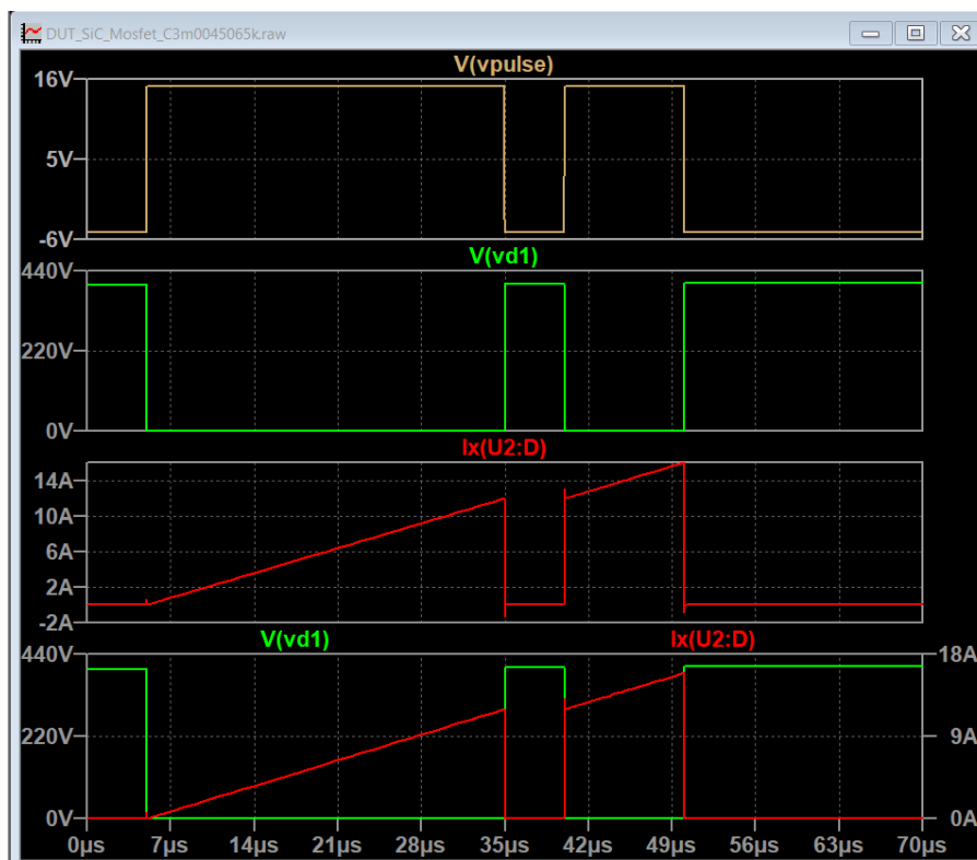
Figure 8. Driving pulses and voltage, current, and power curves for the C3M0045065K silicon carbide transistor.
