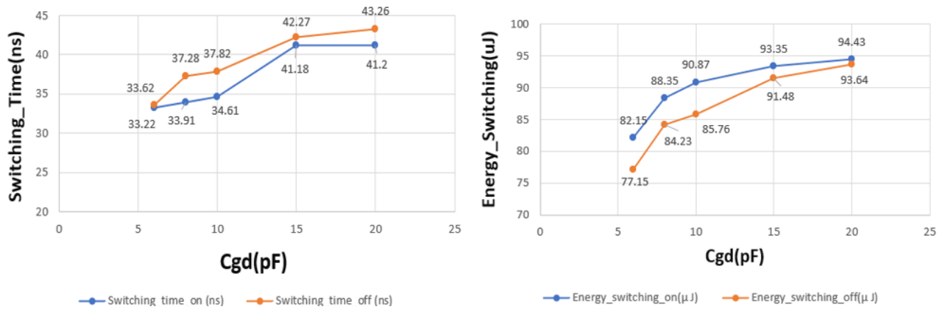
Figure 25. Switching Time Delay and Energy Losses during Turn on/off for Different Cgd.
