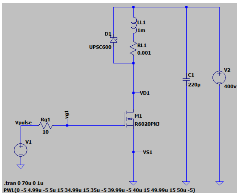
Figure 5. Electrical diagram of the double pulse test circuit on the R6020PNJ silicon transistor.
