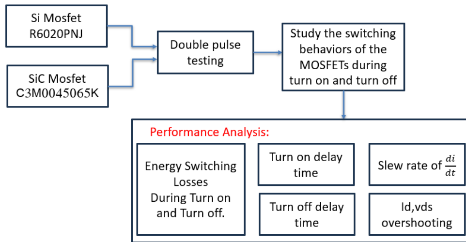
Figure 4. Block diagram of double pulse Testing.
