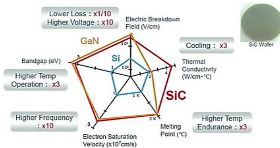
Figure 1. Features of GaN and SiC Mosfets compared to Si Mosfets [14].
