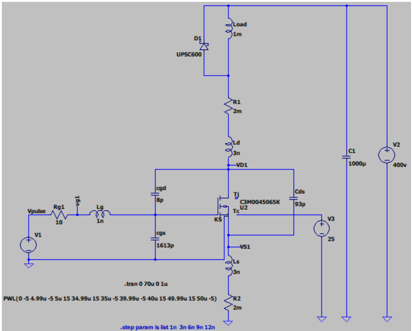
Figure 12. Double pulse Testing for Sic Mosfet under different Values of parasitic Components.
