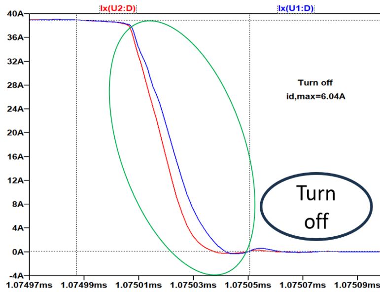
Figure 32. Simulation diagram of dynamic current imbalance at turn-off moment.
