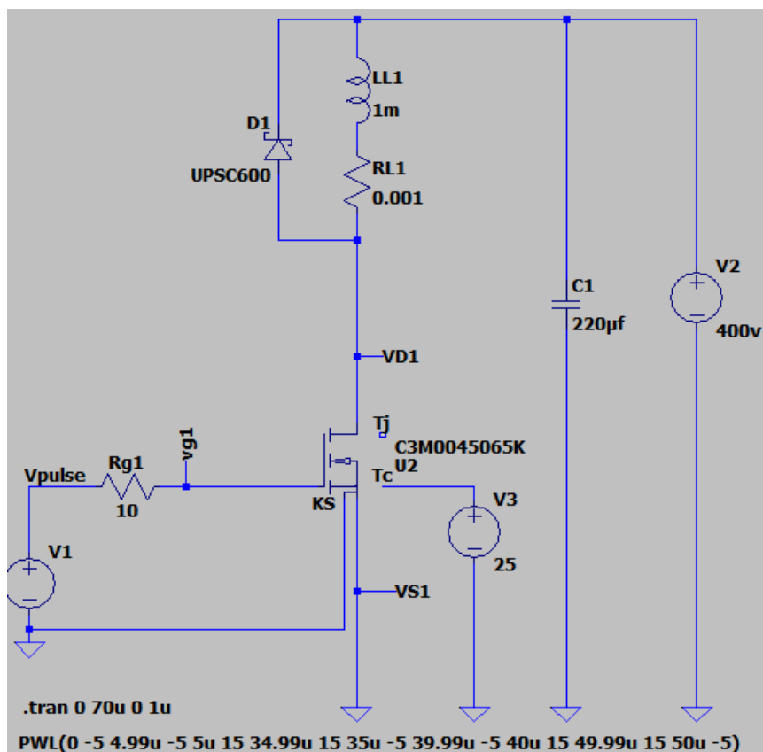
Figure 7. Electrical diagram of the dual pulse test circuit on a silicon carbide transistor C3M0045065K.
