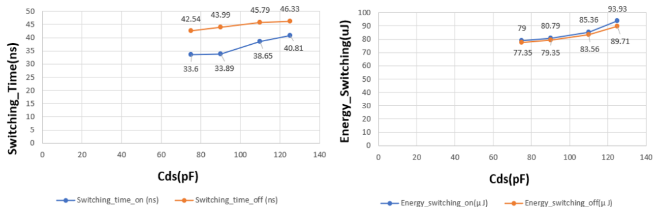
Figure 27. Switching Time Delay and Energy Losses during Turn on/off for Different Cds.
