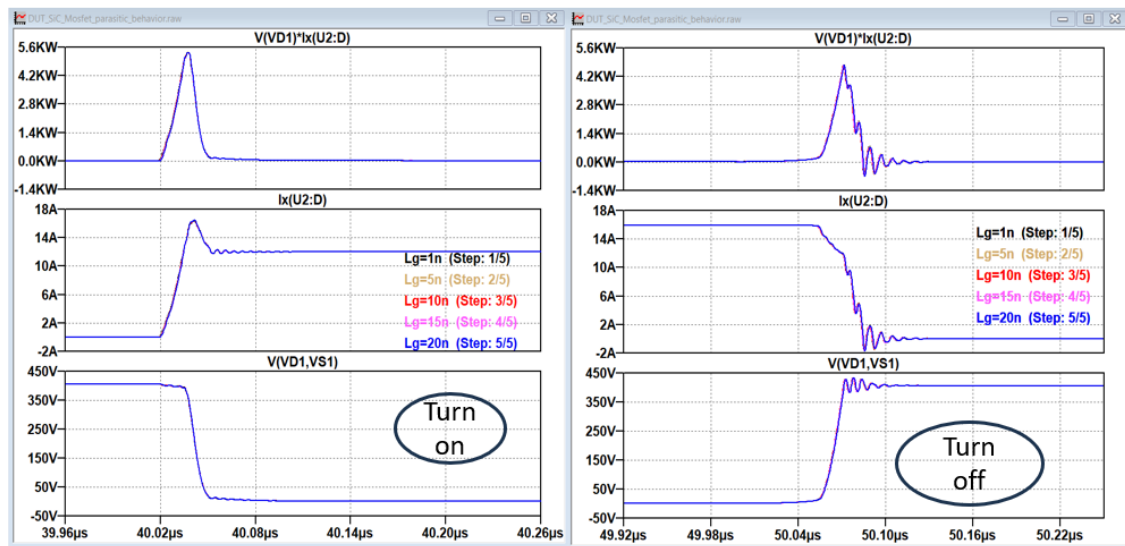
Figure 21. Voltage, current and power loss curves of the transistor during switching (on/off) operation for different L_g values.
