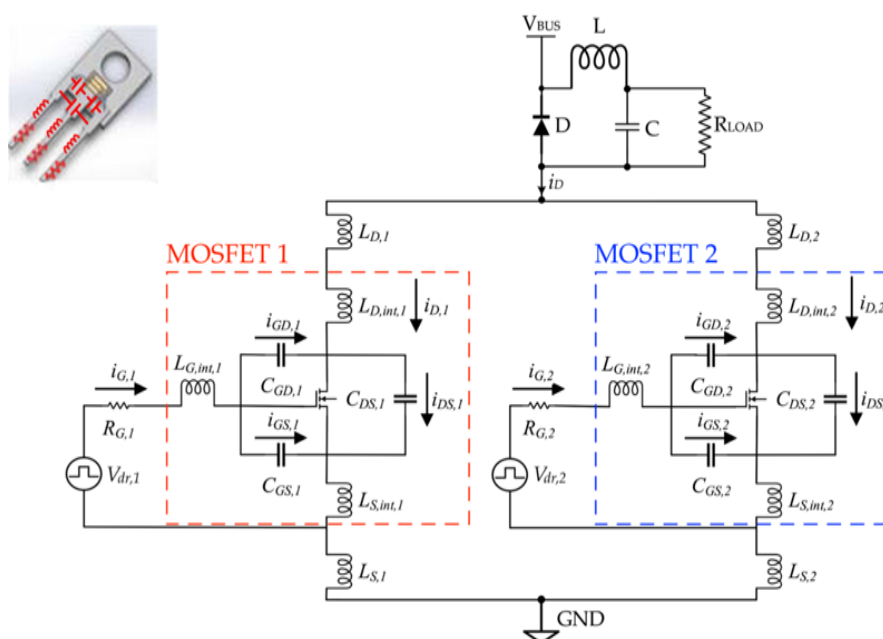
Figure 28. Parallel driving of silicon carbide Mosfets. [1].
