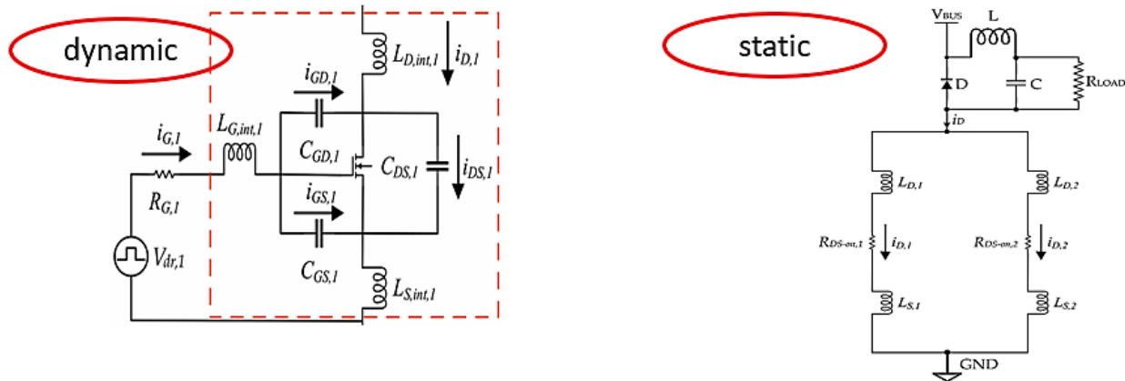
Figure 2. Factors affecting the process of controlling the performance of the switching process and balancing currents between transistors - Static and Dynamic States. [6].
