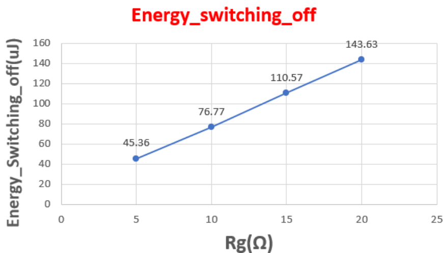
Figure 15. Energy Switching Losses during Turn off for Different R_g Values.
