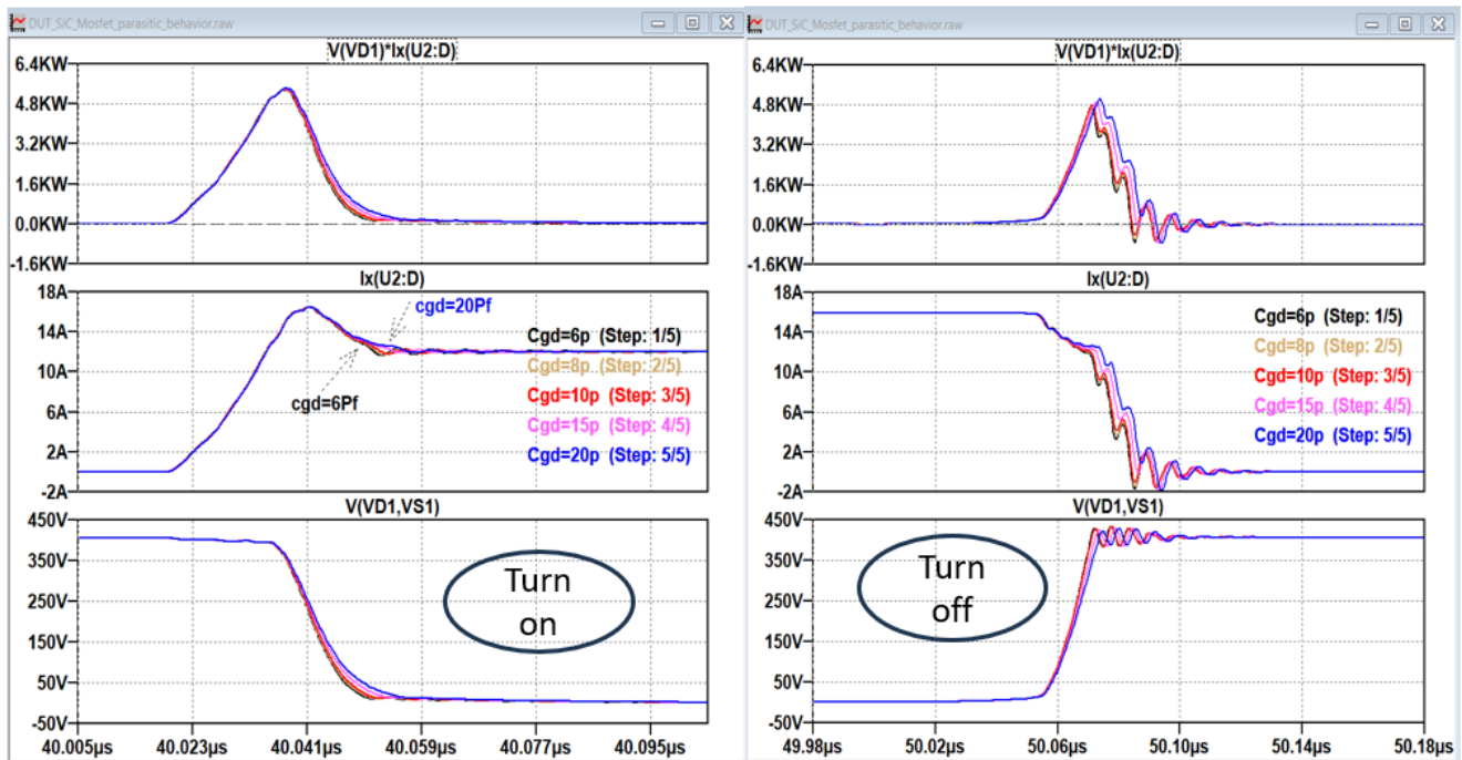
Figure 24. Voltage, current and power loss curves of the transistor during switching (on/off) operation for different C_{gd} values.
