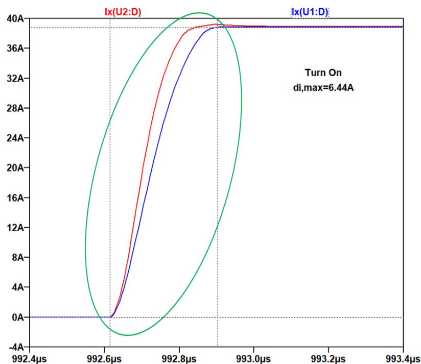
Figure 31. Simulation diagram of dynamic current imbalance at turn-on moment.
