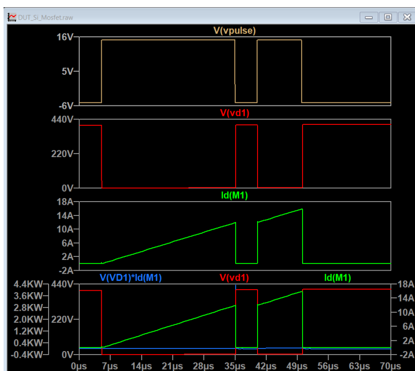
Figure 6. Driving pulses and voltage, current and power curves for the R6020PNJ silicon transistor.
