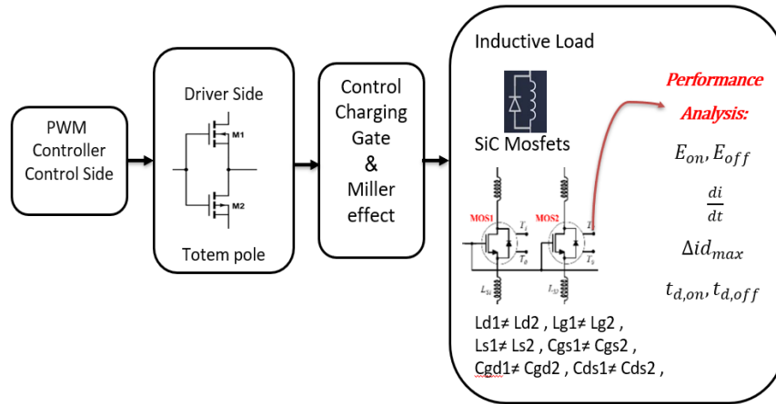
Figure 29. The block diagram of the parallel driving circuit.
