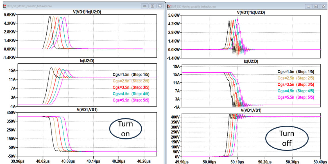
Figure 22. Voltage, current and power loss curves of the transistor during switching (on/off) operation for different C_{gs} values.
