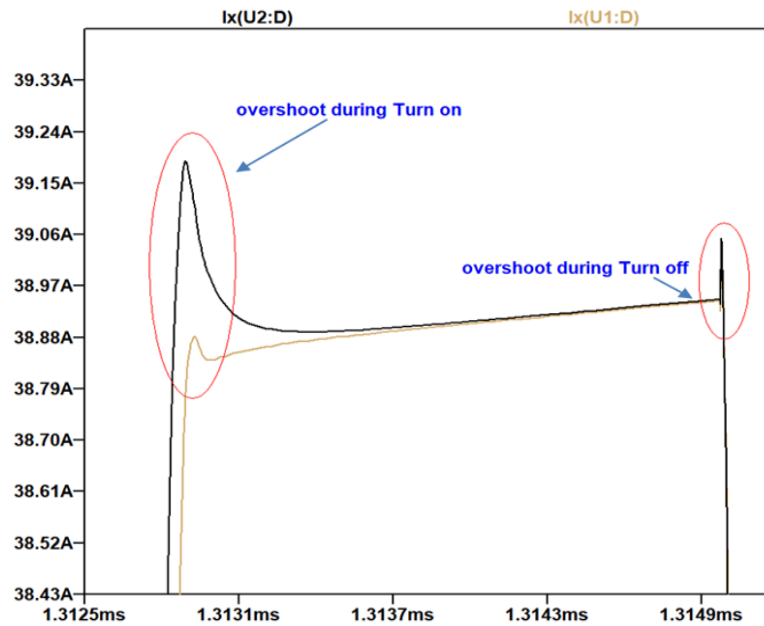
Figure 33. Simulation diagram of Overshooting dynamic current at turn-on/off moment.
