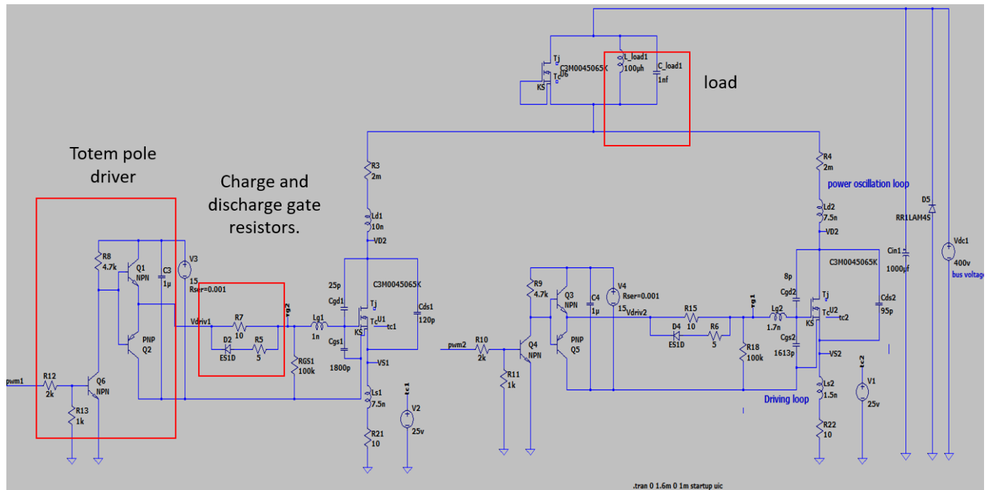
Figure 30. Circuit diagram for driving two C3M0045065K silicon carbide transistors in parallel.
