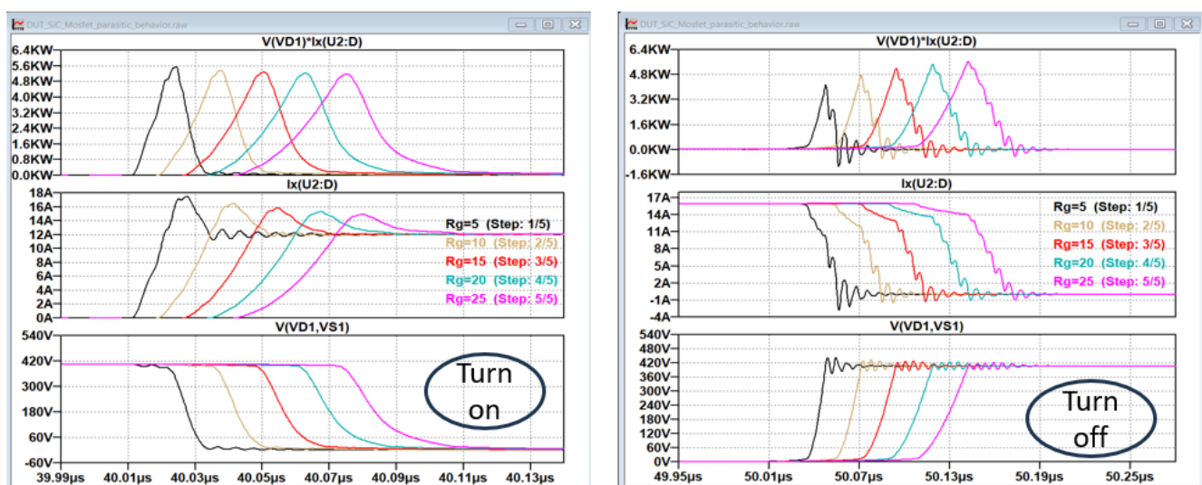
Figure 13. Voltage, current and power loss curves of the transistor during switching (on/off) operation for different R_g values.
