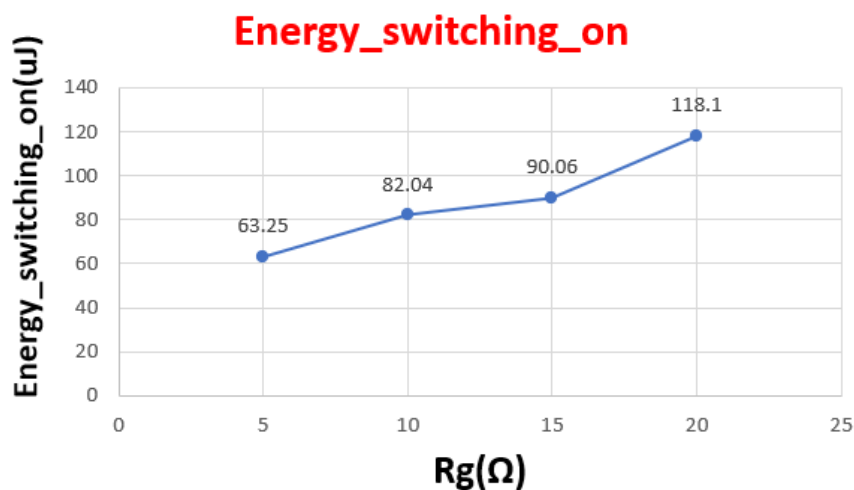
Figure 14. Energy Switching Losses during Turn on for Different R_g Values.
