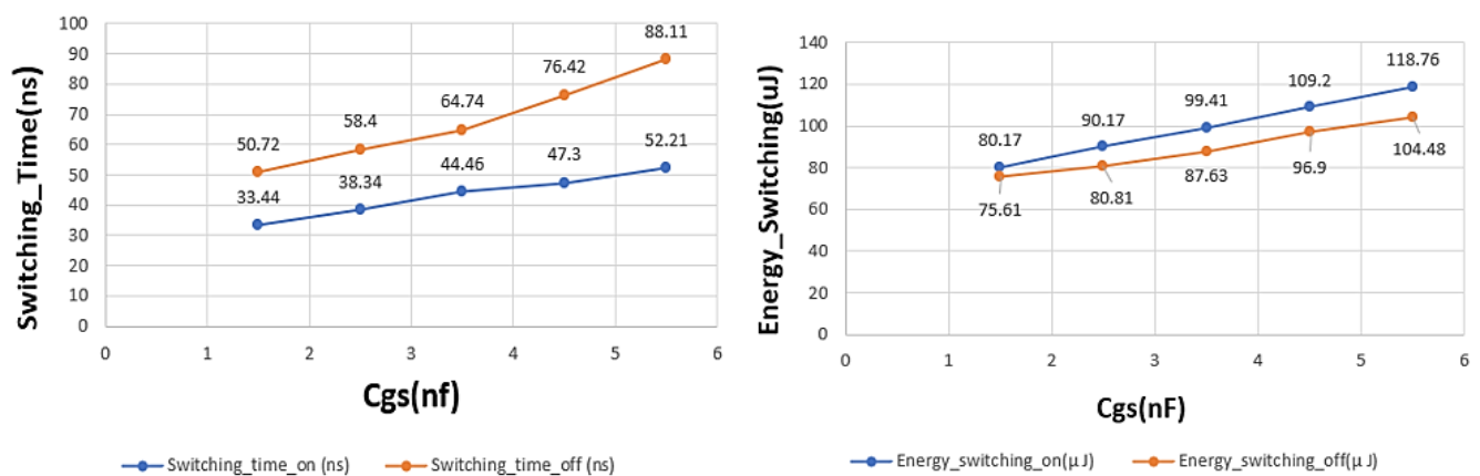
Figure 23. Switching Time Delay and Energy Losses during Turn on/off for Different C_{gs} .
