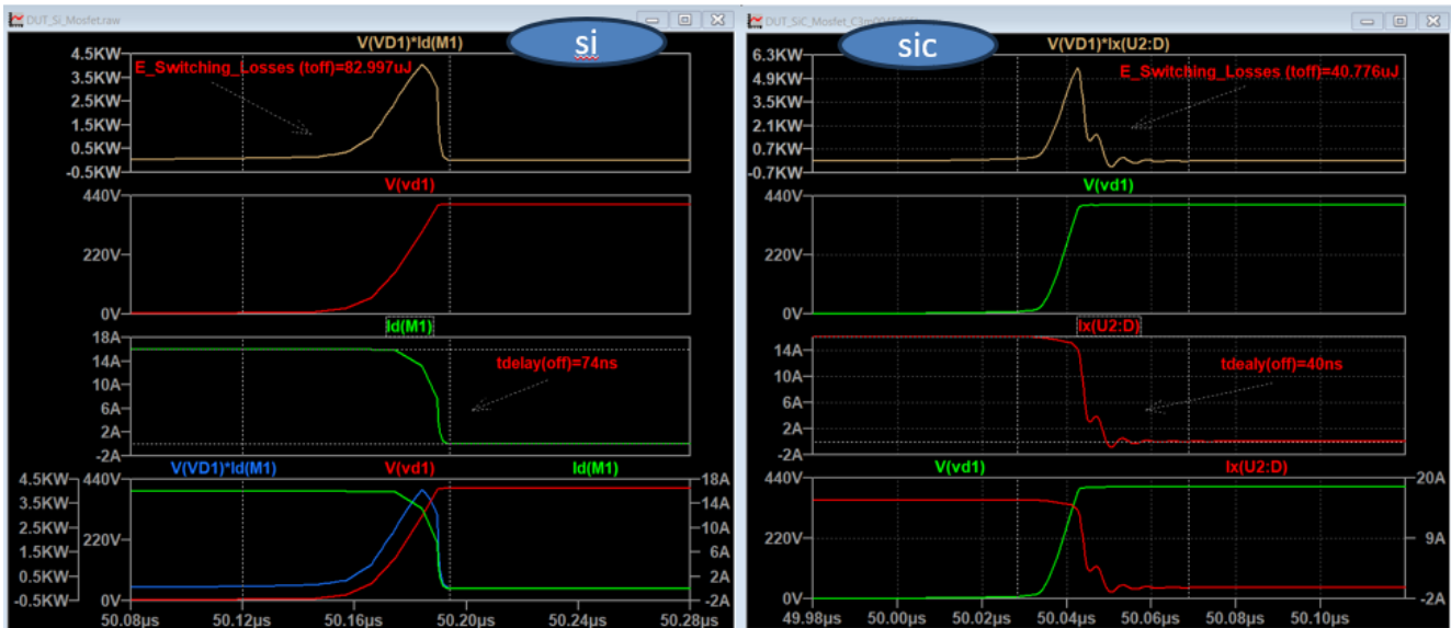
Figure 10. Voltage, current and power loss curves of the two transistors during Turn off operation.
