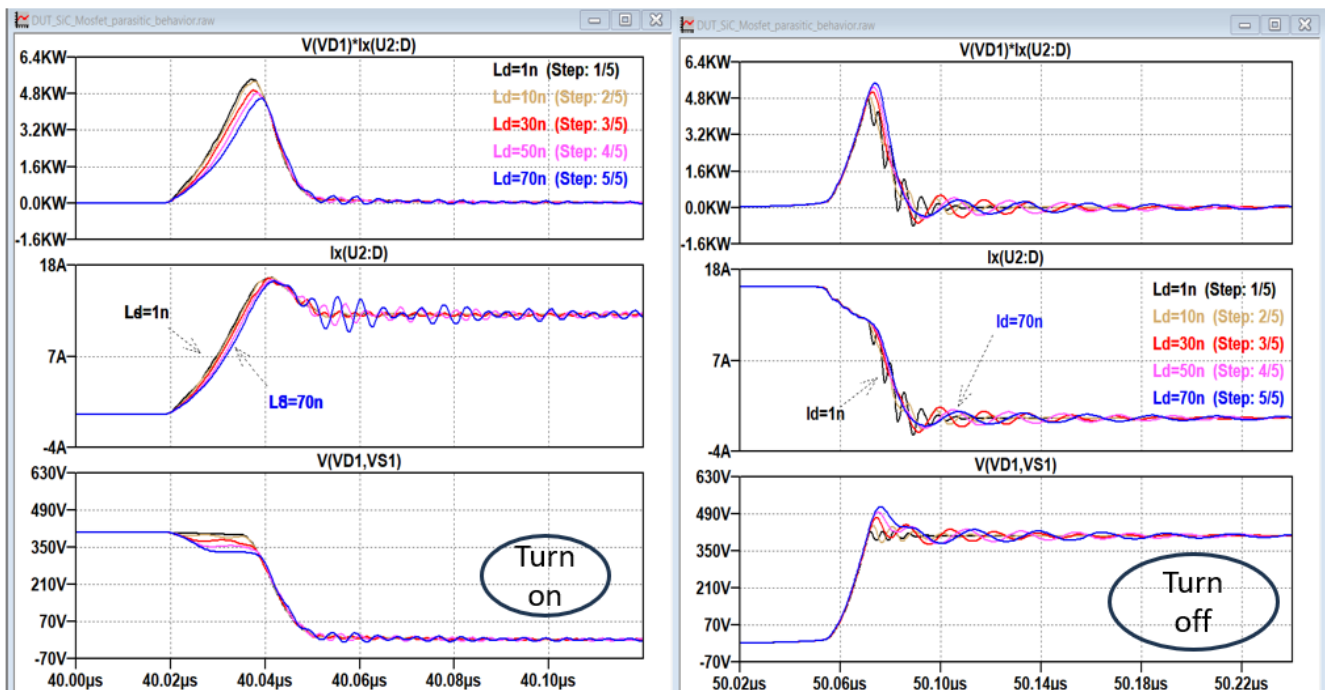
Figure 19. Voltage, current and power loss curves of the transistor during switching (on/off) operation for different L_d values.
