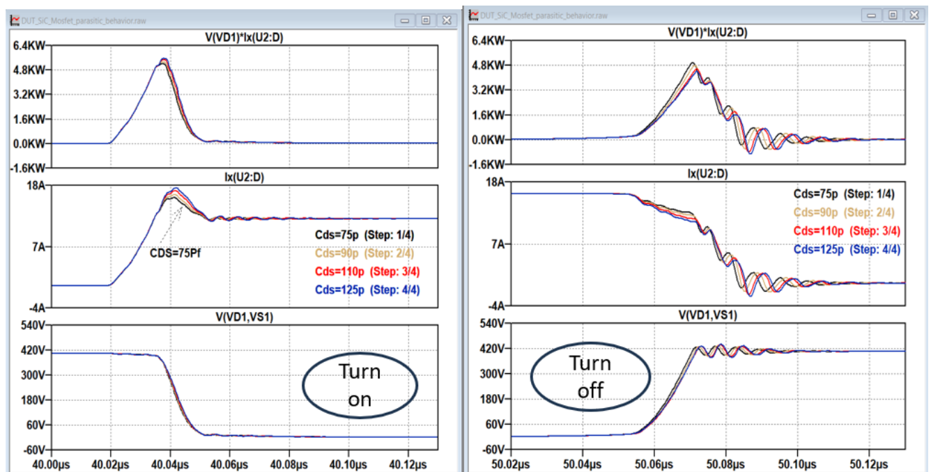
Figure 26. Switching Time Delay and Energy Losses during Turn on/off for Different Cds.
