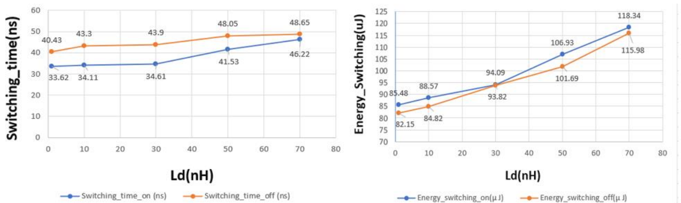
Figure 20. Switching Time Delay and Energy Losses during Turn on/off for Different L_d Values.
