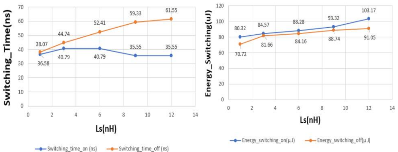
Figure 18. Switching Time Delay and Energy Losses during Turn on/off for Different L_s Values.
