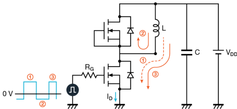
Figure 3. Double pulse test mechanism [15].
