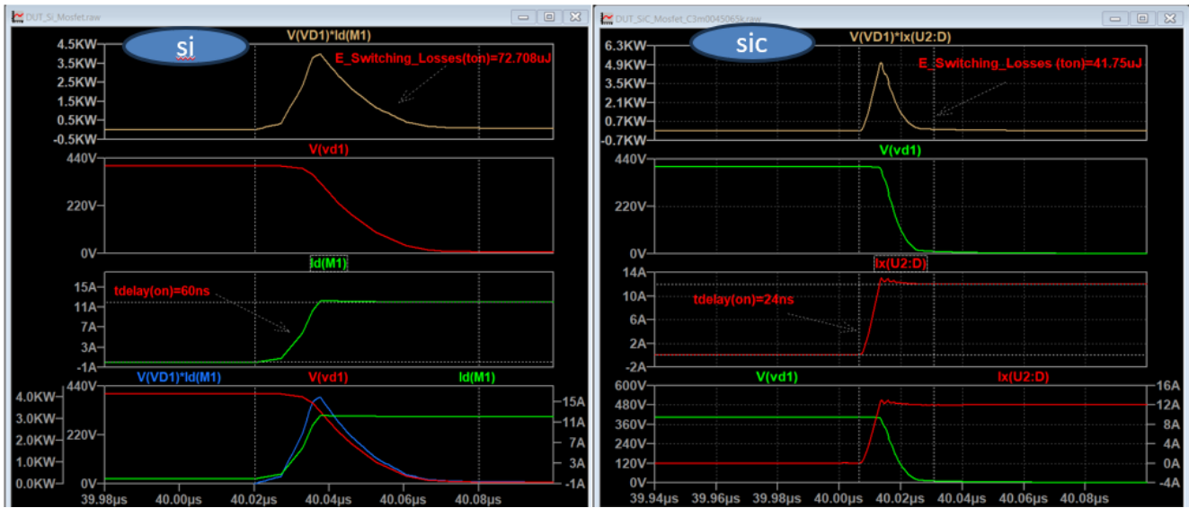
Figure 9. Voltage, current and power loss curves of the two transistors during Turn on operation.
