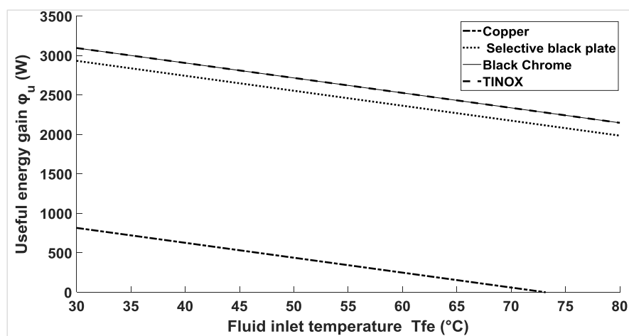
Figure 6. Influence of the coating on the useful energy gain as a function of the heat transfer fluid inlet temperature.
