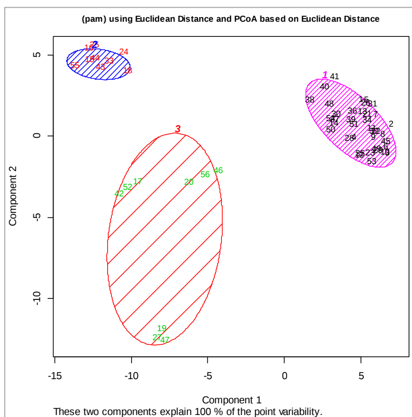
Figure 5. Partitioning around methods using Euclidean distance and PcoA.
