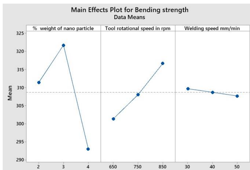
Figure 8. Main effect plot for bending strength.
