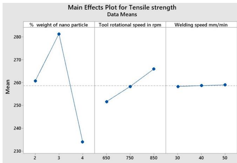
Figure 7. Main effect plot for tensile strength.
