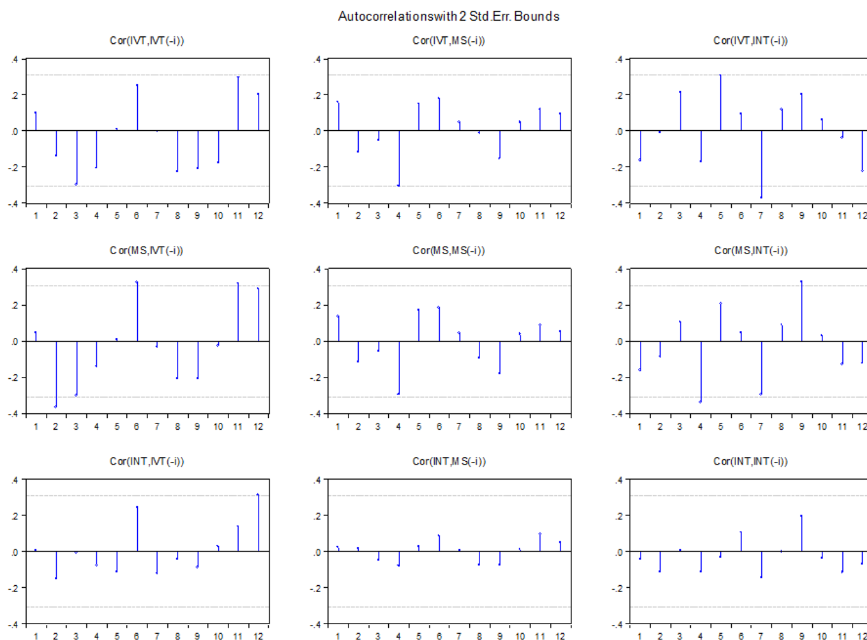
Figure 3. Autocorrelation with 2 std Err. Bounds.
