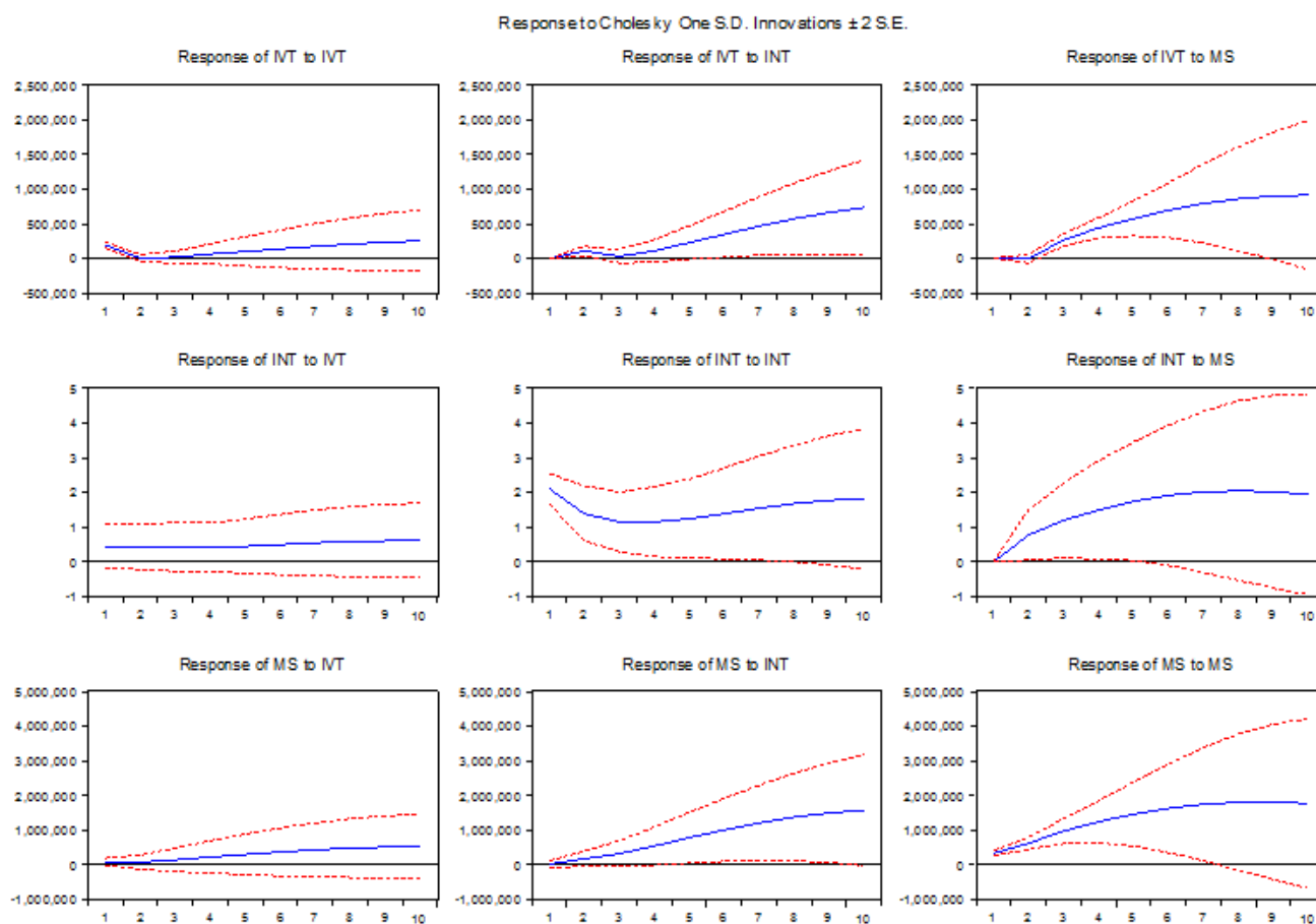
Figure 1. VAR system impulse response function (IRF) analysis.
