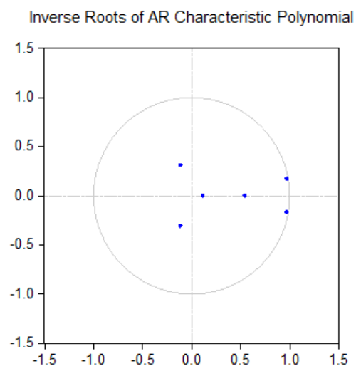
Figure 2. Inverse Roots Characteristic Polynomial.
