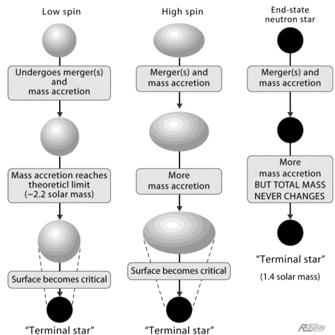
Figure 2. Consequences of further mass acquisition through mergers, collisions, and/or gradual accretion, for the three types of neutron stars. This is a continuation of the flowchart that begins in Figure 1. Low-spin neutron stars remain more or less spherical, which means their surface area is minimal in proportion to volume, which in turn means that the surface becomes critical much sooner than it would if it had the ovate shape associated with a high rate of rotation. While the mass limit for low-spin neutron stars is about 2.2 M_{\odot} , the corresponding limit for high-spin neutron stars exceeds 3.3 M_{\odot} . Categorically, End-State neutron stars are unique. Regardless of the quantity of additional mass accrual/absorption, the total mass content never changes, and the volume and radius never changes. Hence, the density never changes. Surface criticality means that the universal space medium (the vacuum) is flowing into the structure's surface at lightspeed. In this evolutionary sequence, lies the explanation of why the vast majority of neutron stars are identical.
