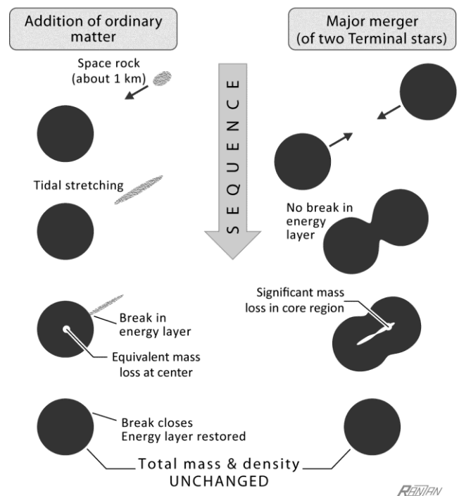
Figure 5. Matter extinction, a mass loss process resulting from aether deprivation, occurs during gravitational mergers and mass encounters. The schematic sequences show the main features of the mechanism by which Terminal stars maintain their total-mass invariance—their constant quantity of matter—regardless of any accretion rate. As 'new' matter falls in, 'old' matter vanishes at the core (shown in cross section). What is not shown are the polar emission beams through which great surges and bursts of energy (derived mainly from infalling-mass-to-energy conversion) are emitted during mass accrual.
