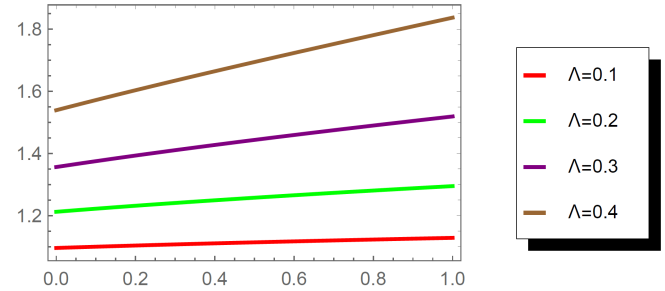
Figure 12. For varying of \lambda = 4 and b(t) = 5 , the variation of \Delta_a with regards ' r' ' and ' \Lambda' '
