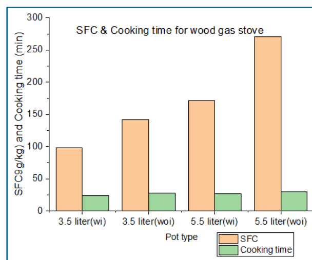
Figure 6. The SFC and cooking time versus pot types for WGS.
