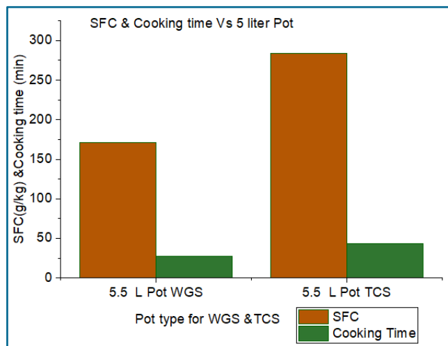
Figure 8. The SFC and cooking time versus pot types.
