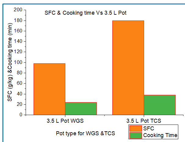
Figure 7. The SFC and cooking time VS pot types for WGS & TCS.
