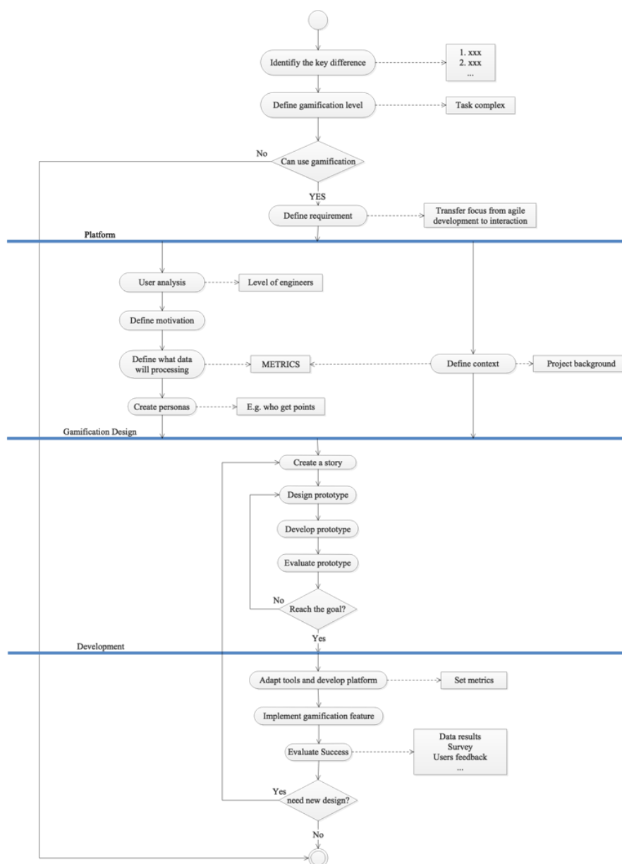
Figure 1. S2S-G Framework.
