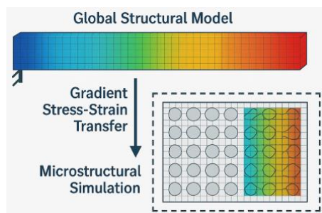
Figure 11. Multiscale Simulation of a Composite Beam with Microstructural RVE Integration.
