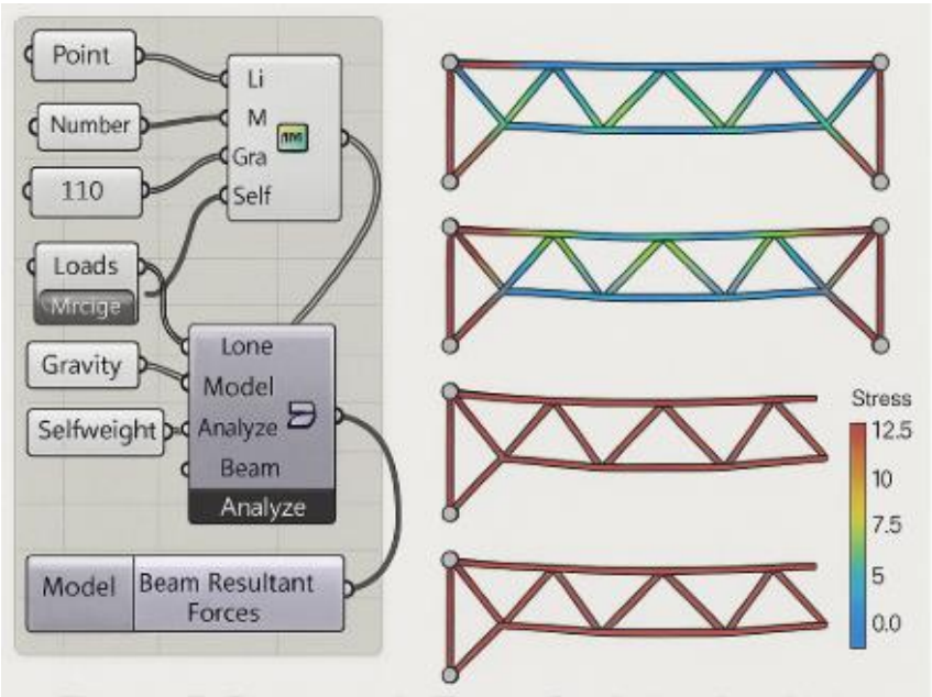
Figure 12. Parametric Truss Optimization Using Grasshopper and Karamba3D.
