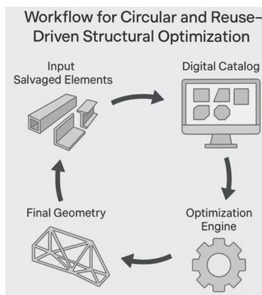
Figure 14. Workflow for Circular and Reuse-Driven Structural Optimization.
