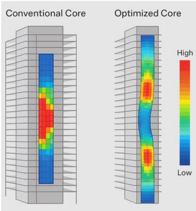
Figure 13. Optimized vs. Conventional Core Layout in a High-Rise Building.
