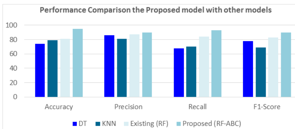
Figure 4. Performance comparison of the crime prediction models.
