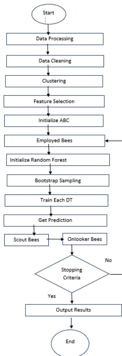
Figure 3. Flow Chart of the Proposed Model (Source: [19]).
