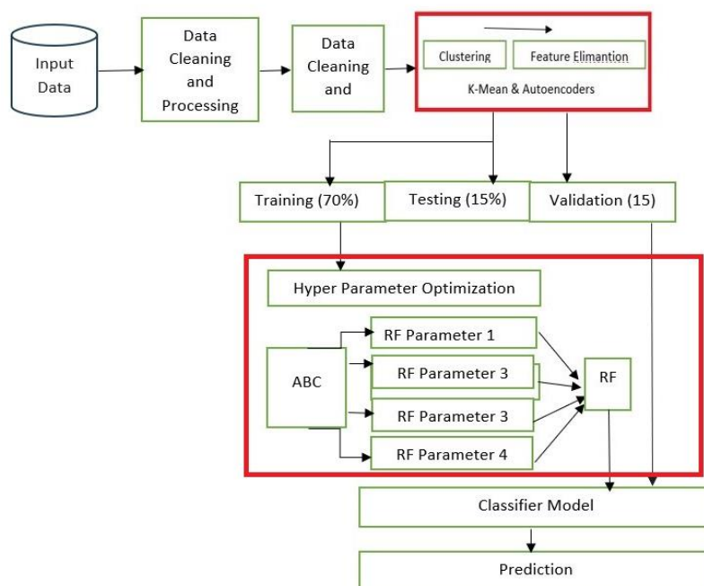
Figure 1. Architecture of the proposed RF- ABC (Source: [19]).
