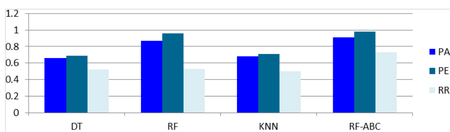
Figure 5. Performance comparison of the performance indices of the crime prediction models.
